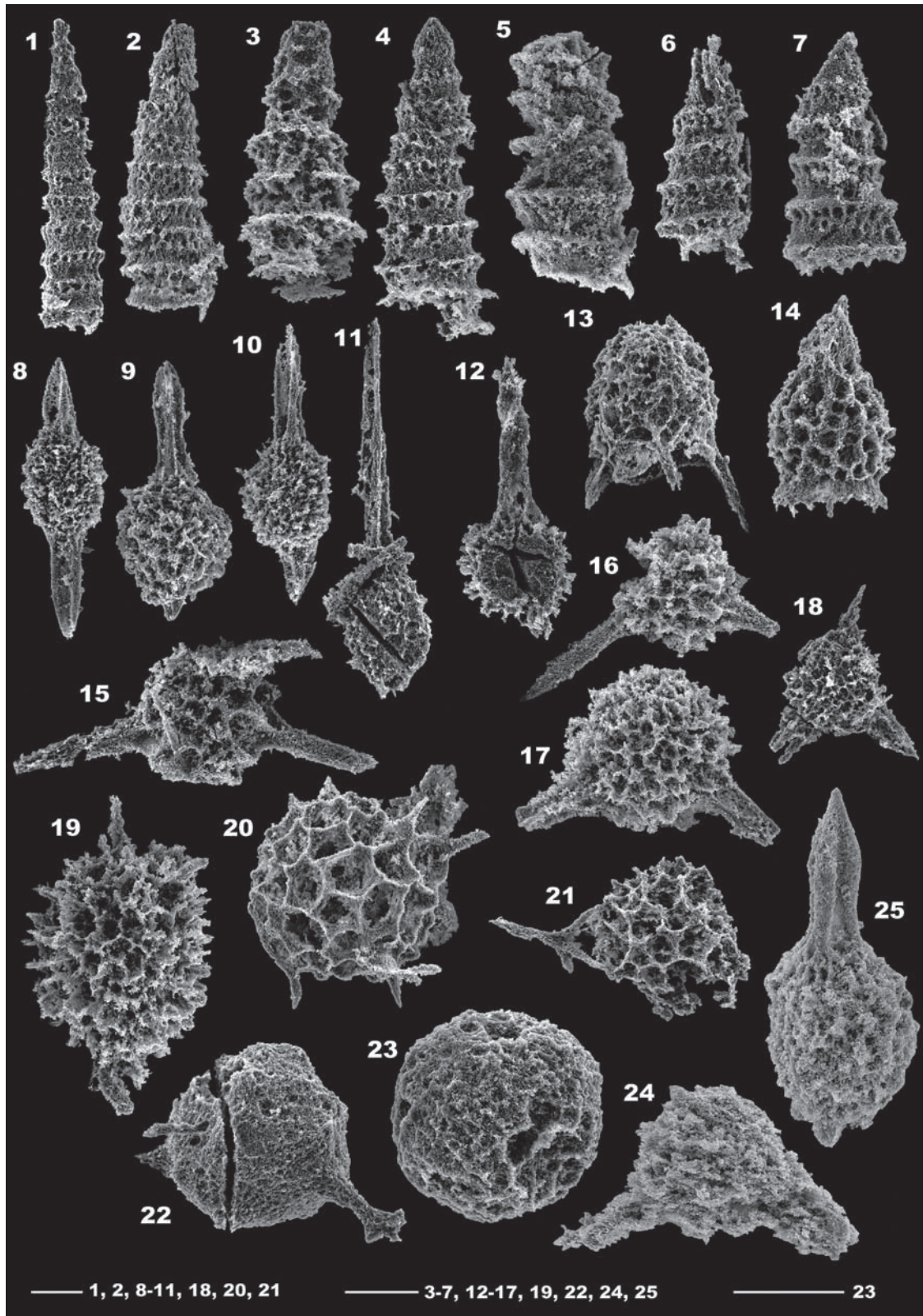
図版3 小沢層のチャート礫から得られた三疊紀放射虫化石(試料2-108,2-26)の電子顕微鏡写真.スケールは0.05mm. 試料2-108 1: Triassocampe sp. A sensu Sugiyama 1997, 2: Triassocampe deweveri (Nakaseko and Nishimura), 3: Triassocampe sp., 4: Triassocampe ? sp. C sensu Yao 1982, 5-7: Triassocampe spp., 8: Pseudostylosphaera japonica (Nakaseko and Nishimura), 9-12: Pseudostylosphaera spp., 13: Hozmadia spp., 14: Yeharaia mascula Sugiyama, 15-17: Betraccium spp., 18: Eptingium sp., 19: Pentactinocarpus fusiformis Dumitrica, 20: Pentactinocarpus awaensis (Nakaseko and Nishimura), 21: Pentactinocarpus sp., 22: Kahlerosphaera sp., 23: Cenosphaera sp. 試料2-26 24: Eptingium sp., 25: Pseudostylosphaera spinulosum (Nakaseko and Nishimura)
